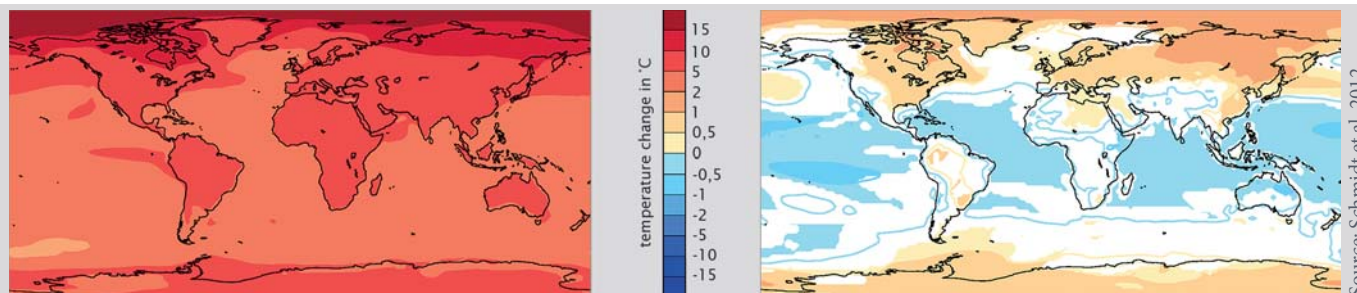
Modelling of temperature changes in the climate scenario with a CO 2 concentration four times higher than the pre-industrial level (left) and in the scenario of the application of RM technologies to maintain the pre-industrial global average temperature despite the high CO 2 concentration (right). A uniform temperature reduction through RM measures would probably not be achievable; the consequence would be overcooling of the tropics and warming of the polar regions.
